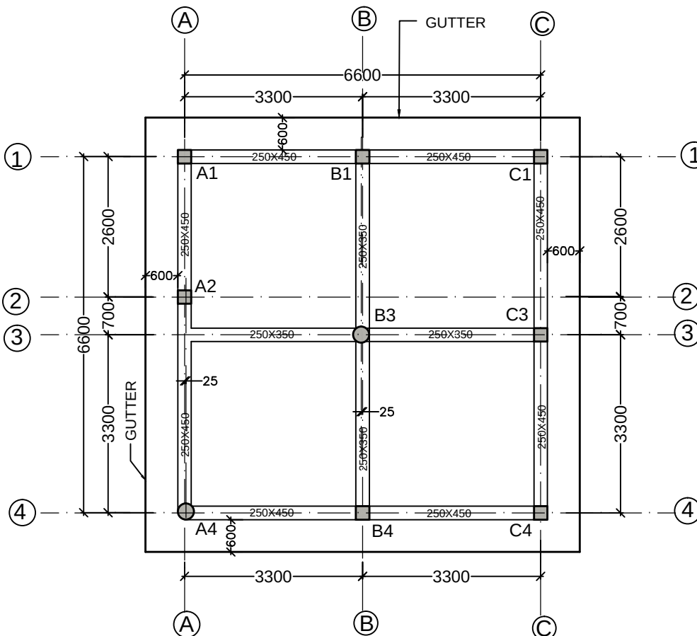
LAYOUT OF POST PLATE BEAM
